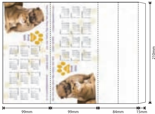
Type A Tent Card Overall Dimension 297mm x 210mm
